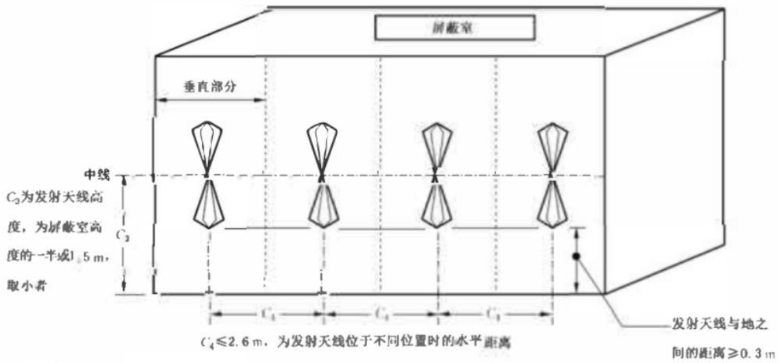
d) 谐振范围测量发射天线布置(垂直极化), 20 MHz~100 MHz
